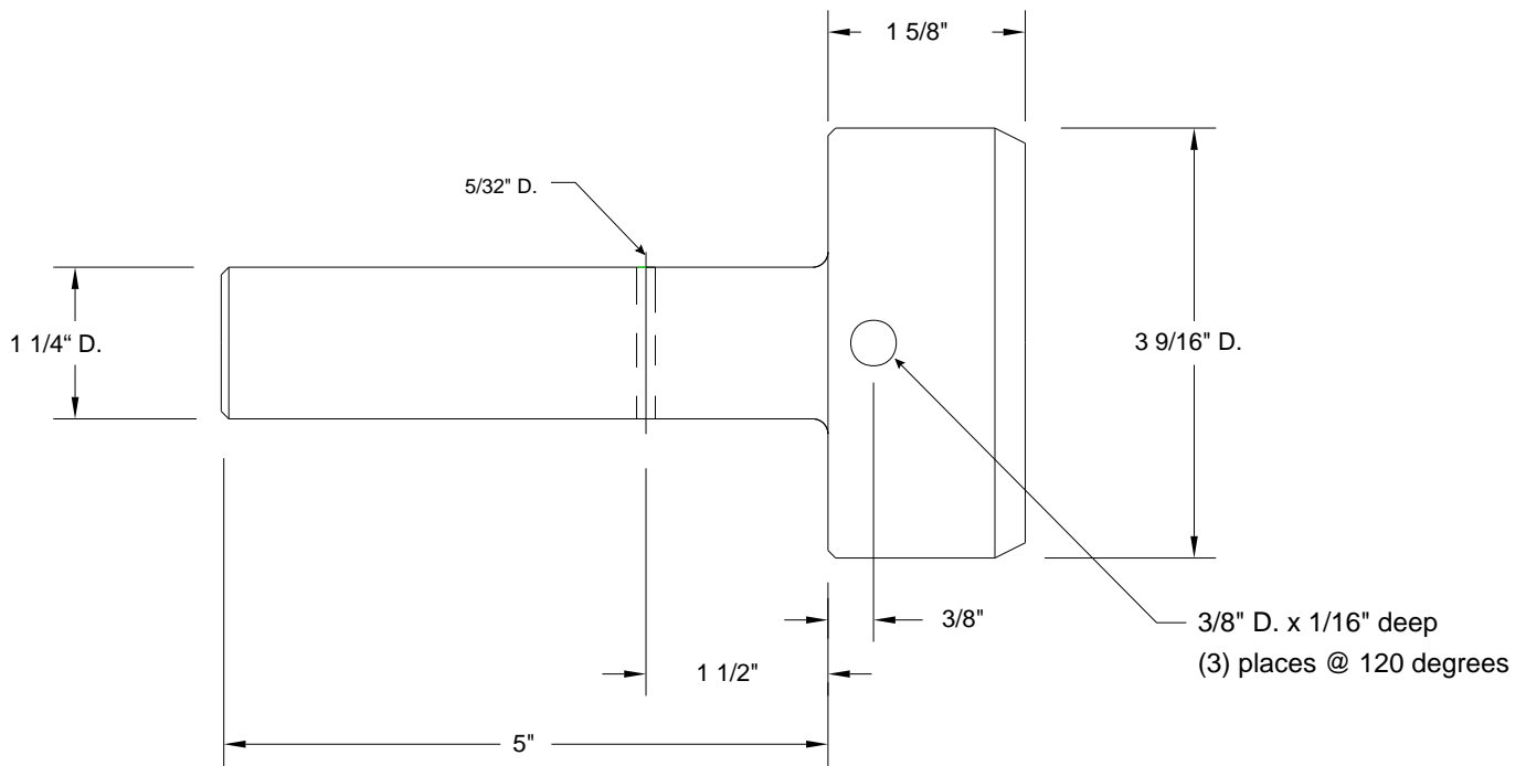
NW 9F Gudgeon, Cross Drilled 1 1/4" x 5" stem, no keyway
